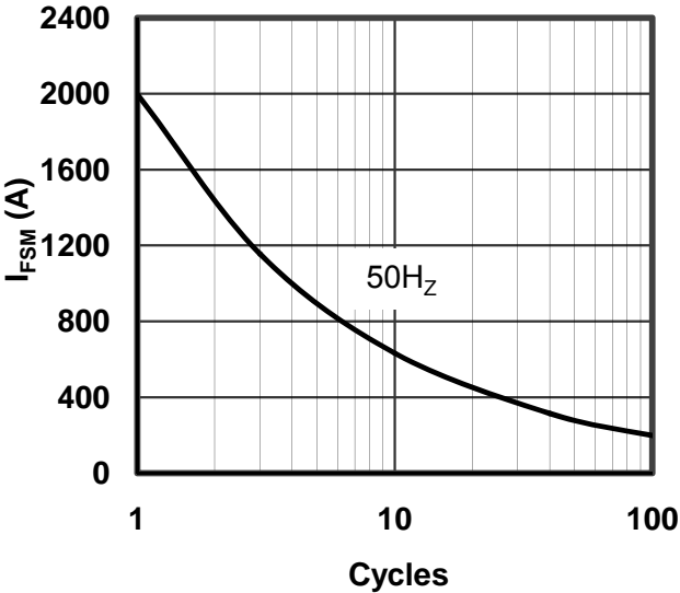
Figure 3. Max Non-Repetitive Forward Surge Current
