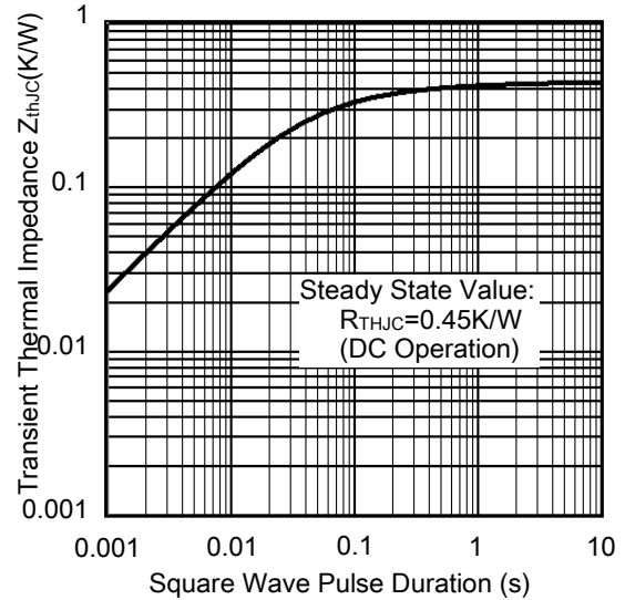
Figure 10. Thermal Impedance Z_{\theta JC} Characteristics
