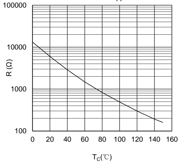
Figure 14. NTC Characteristics
