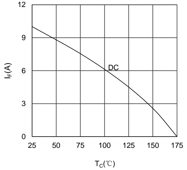
Figure 16. Forward current vs Case temperature Diode-inverter
