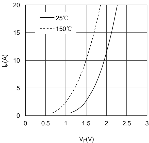
Figure 7. Diode Forward Characteristics Diode -inverter
