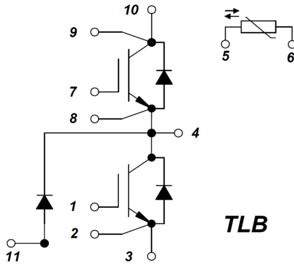
Figure 14. Circuit Diagram
