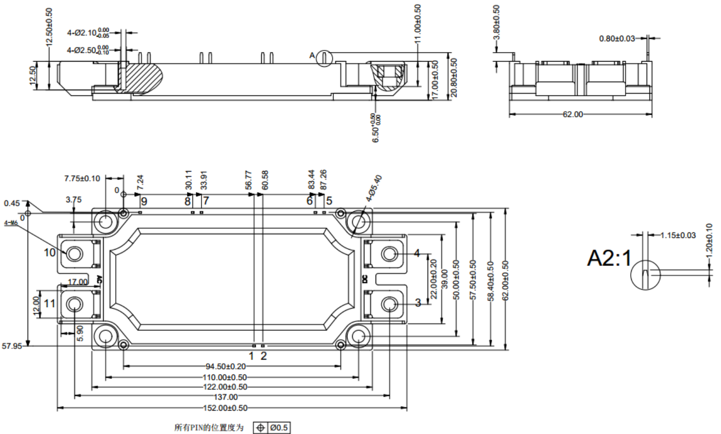
Dimensions in (mm) Figure 15. Package Outline
