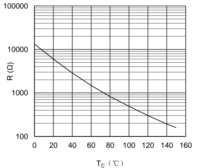
Figure 13. NTC Characteristics
