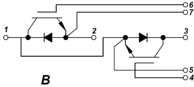
Figure 13. Circuit Diagram
