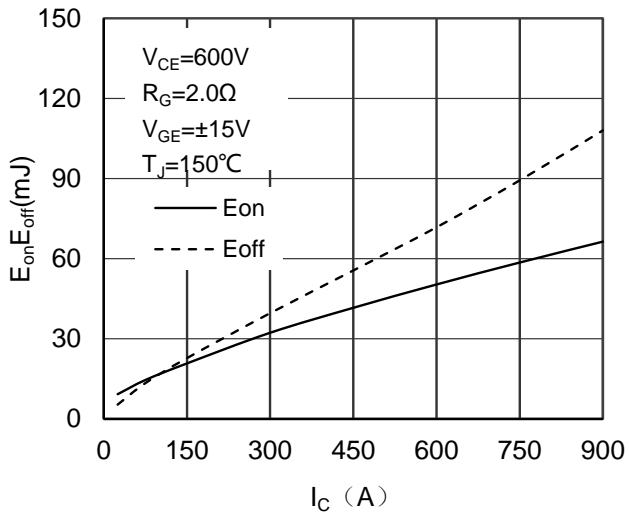
Figure 5. Switching Energy vs Collector Current IGBT-inverter
