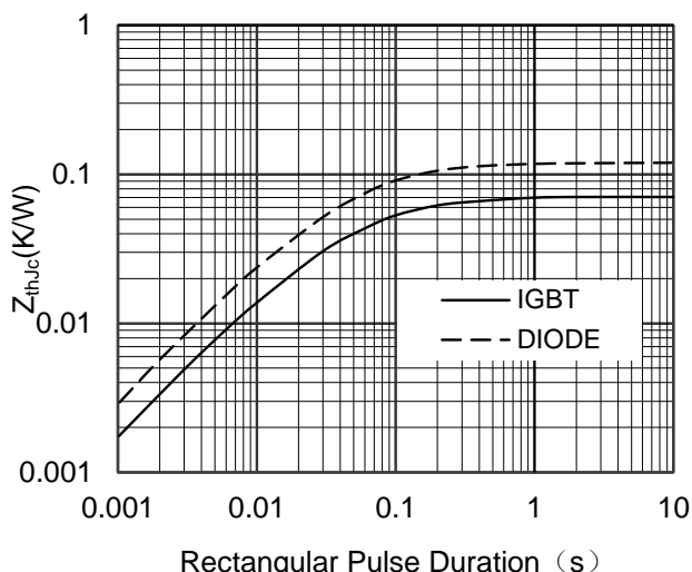
Figure 12. Transient Thermal Impedance of Diode and IGBT-inverter
