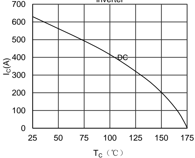
Figure 7. Collector Current vs Case temperature IGBT-inverter
