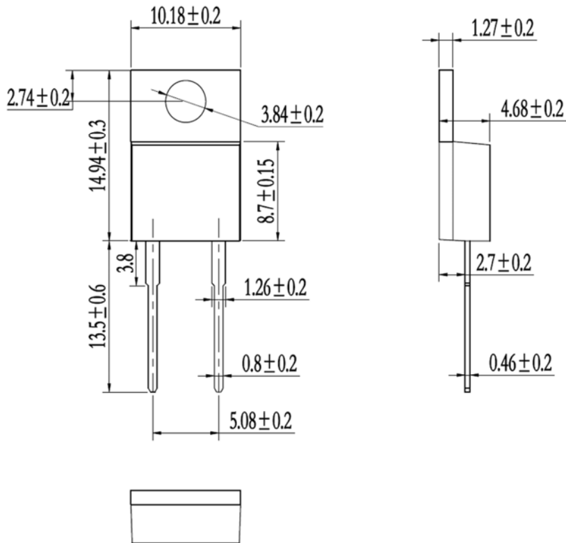
Dimensions in (mm) Figure 8. Package Outline
