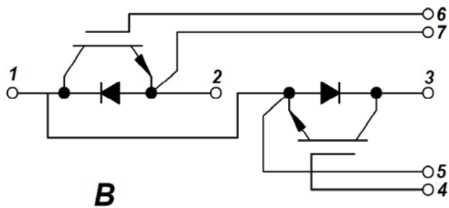
Figure 13. Circuit Diagram
