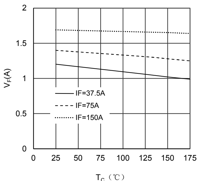
Figure 16. Forward Voltage vs Case temperature
