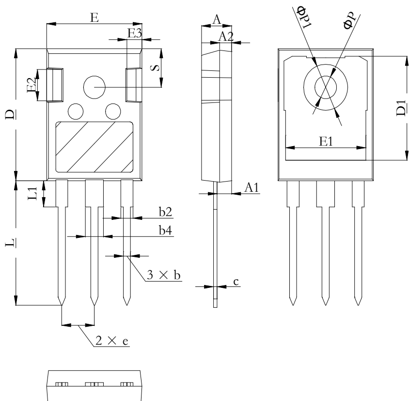
Dimensions in (mm) Figure 21. Package Outline
