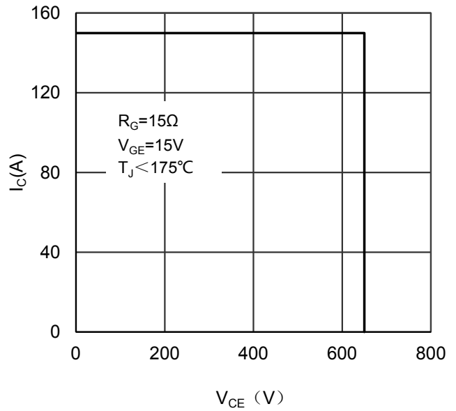
Figure 8. Reverse Biased Safe Operating Area
