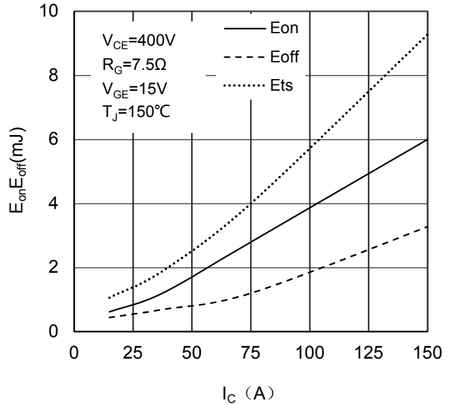
Figure 10. Switching Energy vs Collector Current
