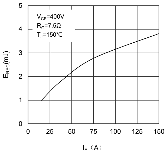
Figure 18. Switching Energy vs Forward Current Diode
