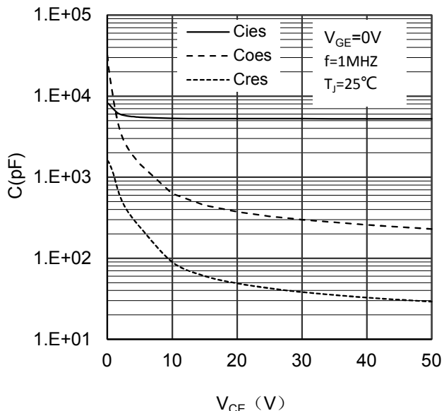
Figure 13. Typical capacitance
