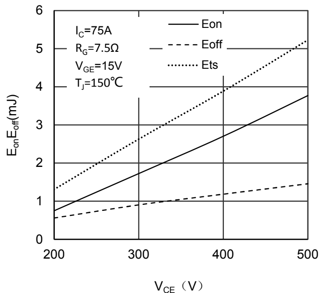
Figure 12. Switching Energy vs Collector-Emitter Voltage
