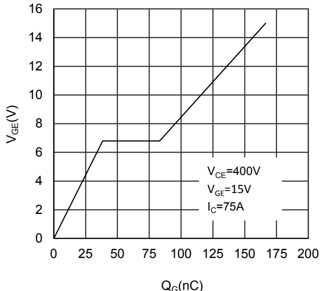
Figure 14. Typical Gate Charge
