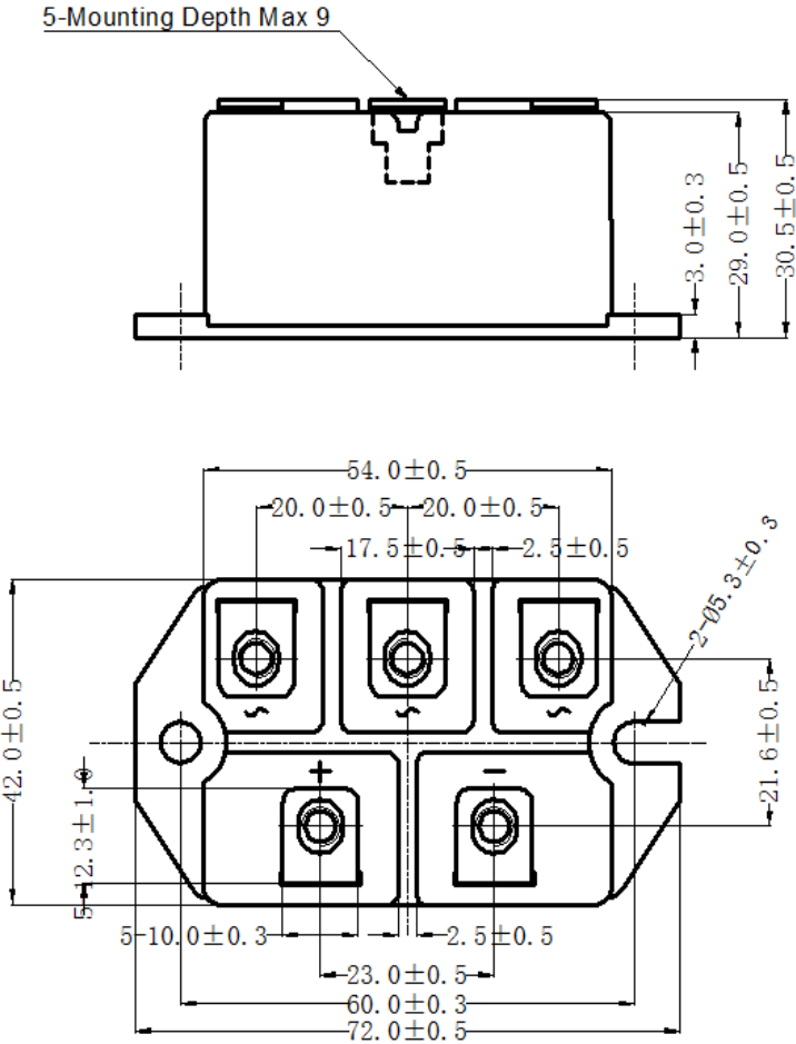
Dimensions in (mm) Figure 6. Package Outline
