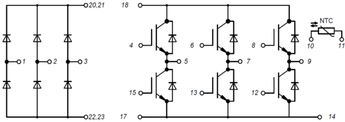
Figure 15. Circuit Diagram
