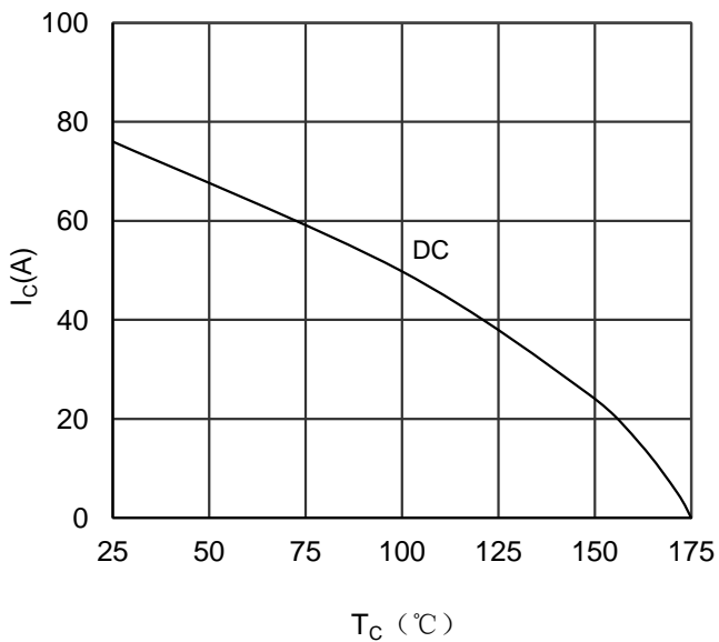
Figure 13. Collector Current vs Case temperature IGBT-inverter
