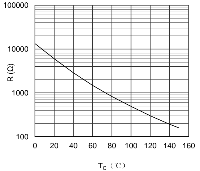
Figure 12. NTC Characteristics
